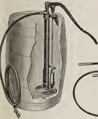
Fig. 832. Outfit A. A small barrel sprayer. 2 gallon per minute at 150 lbs. pressure. Without barrel. Complete with hose and nozzle. $9.50.
